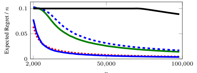
Figure 3. Average regret as n varies with \alpha = 0.1 and \delta = 1/n
